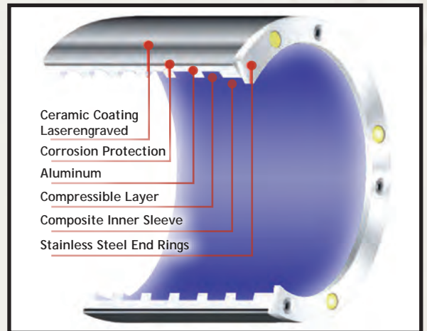
Design of Interflex Anilox-Sleeve
